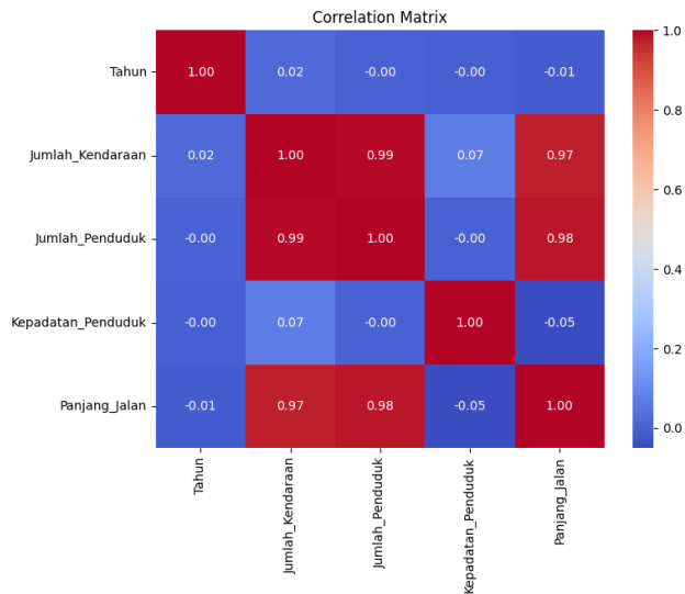
Gambar 1. Correlation Matrix
